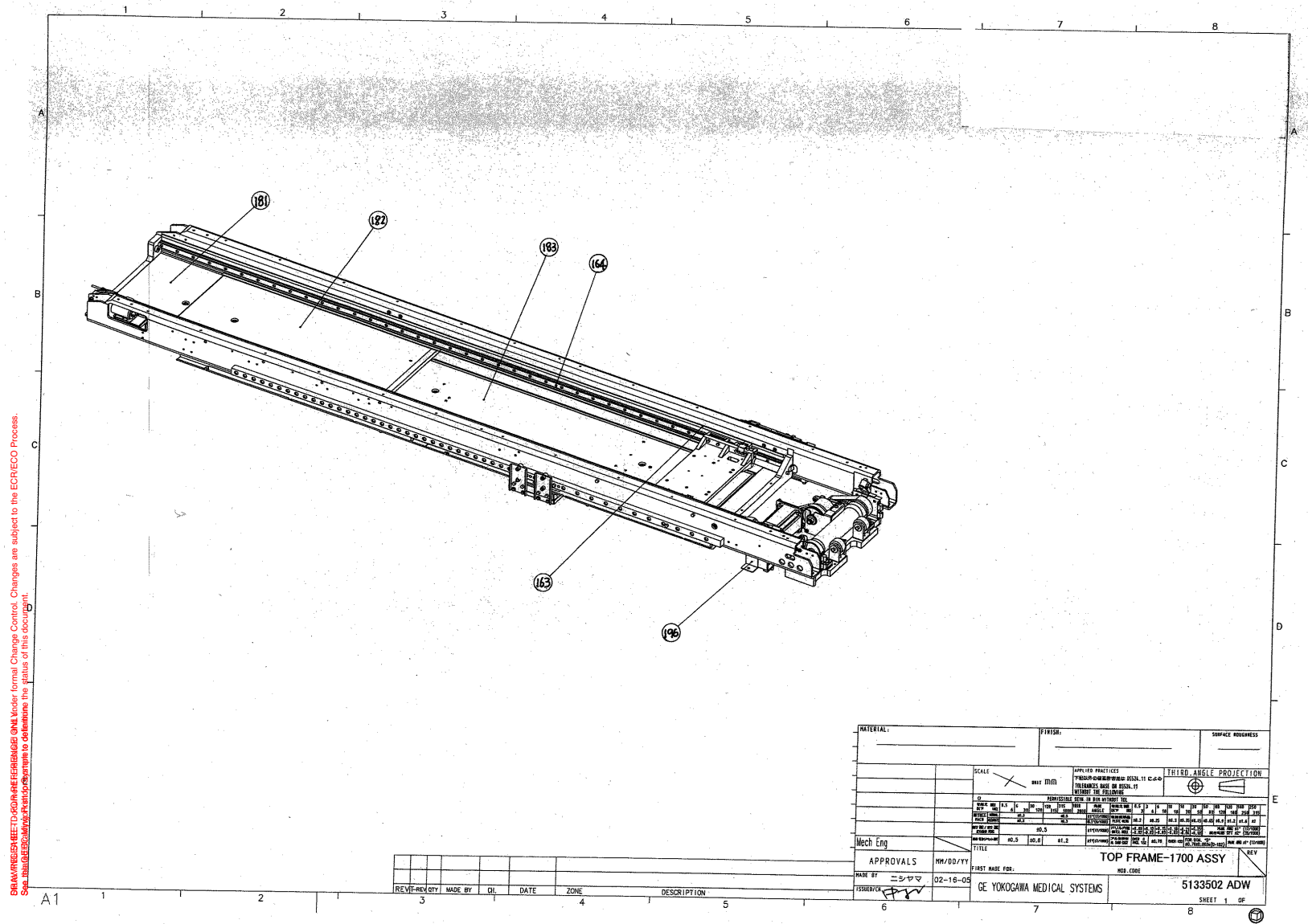
Figure 2-59 Top Frame 1700 Assembly (5133502ADW, sheet 1, rev 5)
