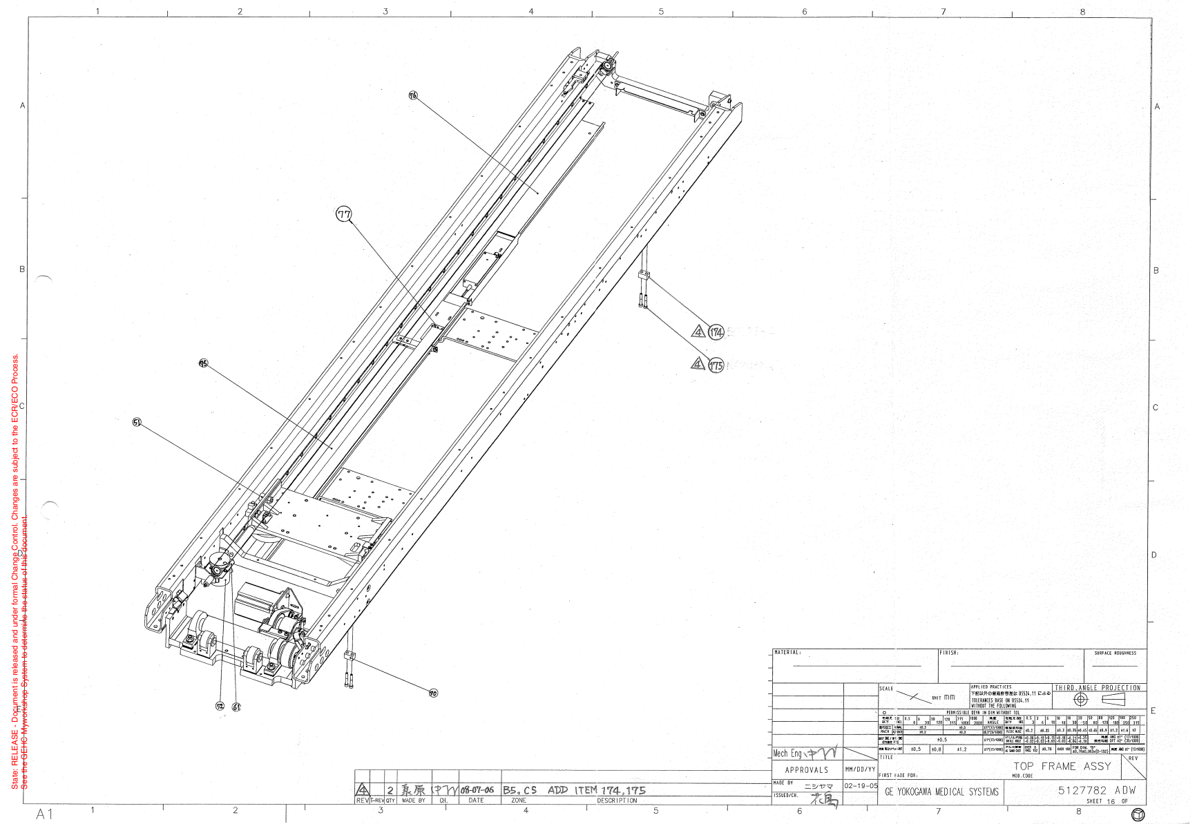
Figure 2-32 Top Frame Assembly (5127782ADW, sheet 16, rev 7)
