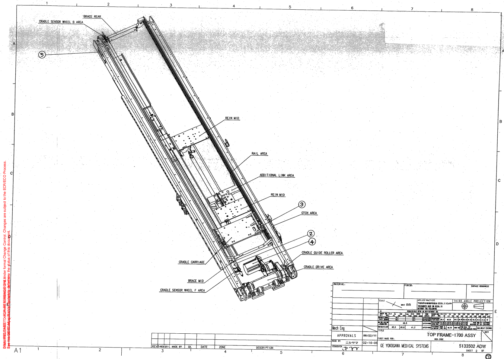
Figure 2-60 Top Frame 1700 Assembly (5133502ADW, sheet 2, rev 5)
