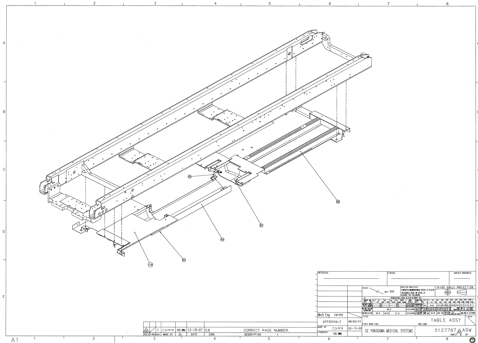
Figure 2-9 Table Assembly (5127787ADW, sheet 9, rev 10)
