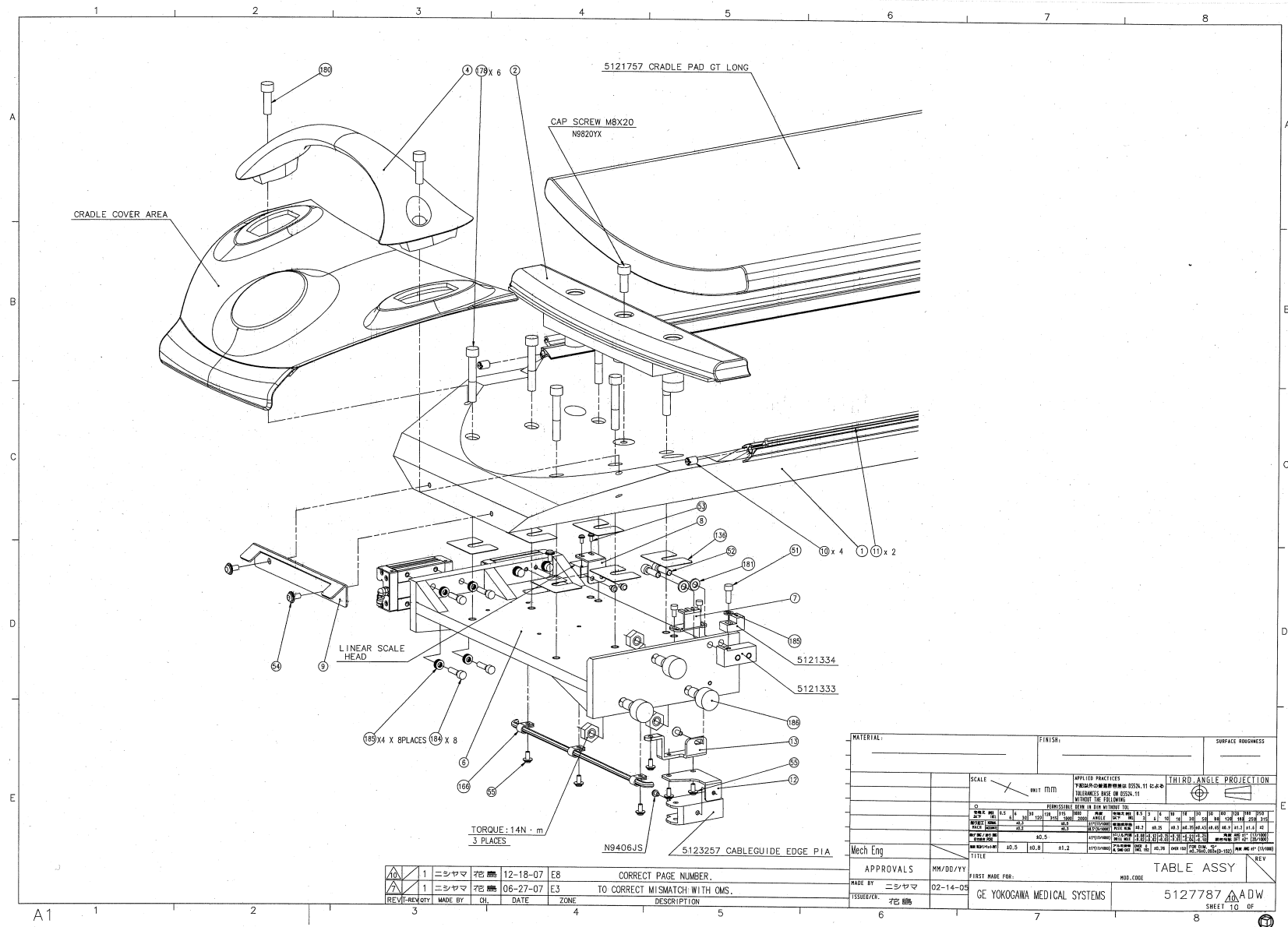
Figure 2-10 Table Assembly (5127787ADW, sheet 10, rev 10)
