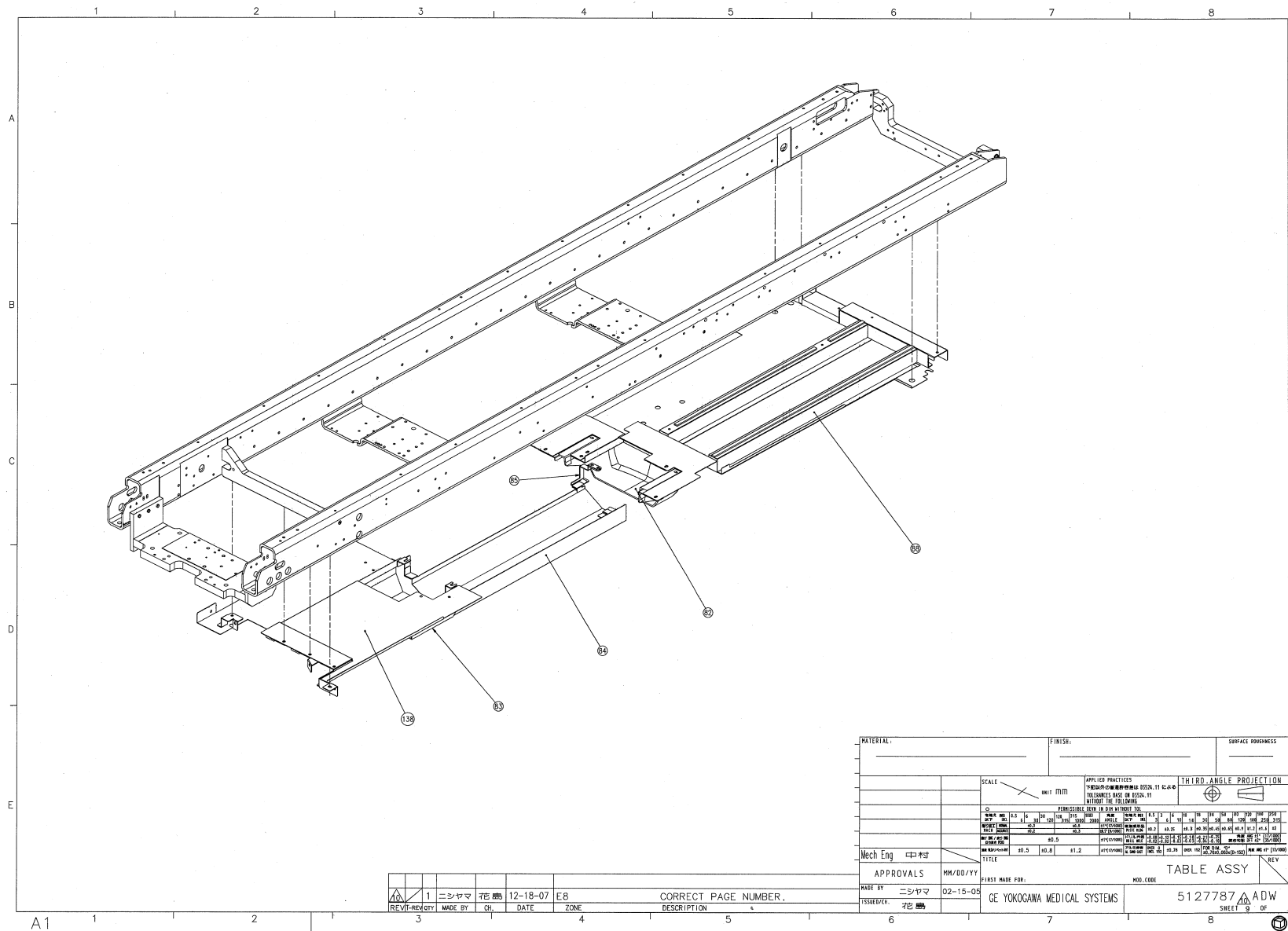
Figure 2-56 Table Assembly (5127787ADW, sheet 9, rev 10)
