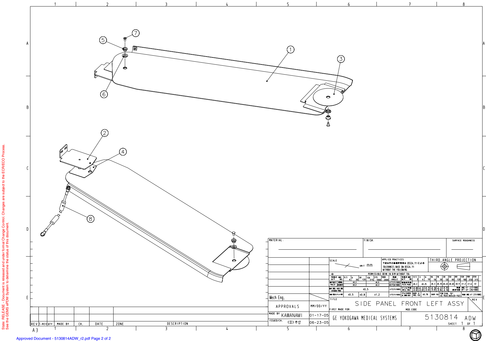
Figure 2-44 Side Panel, Front Left Assembly (5130814ADW, sheet 1, rev 2)
