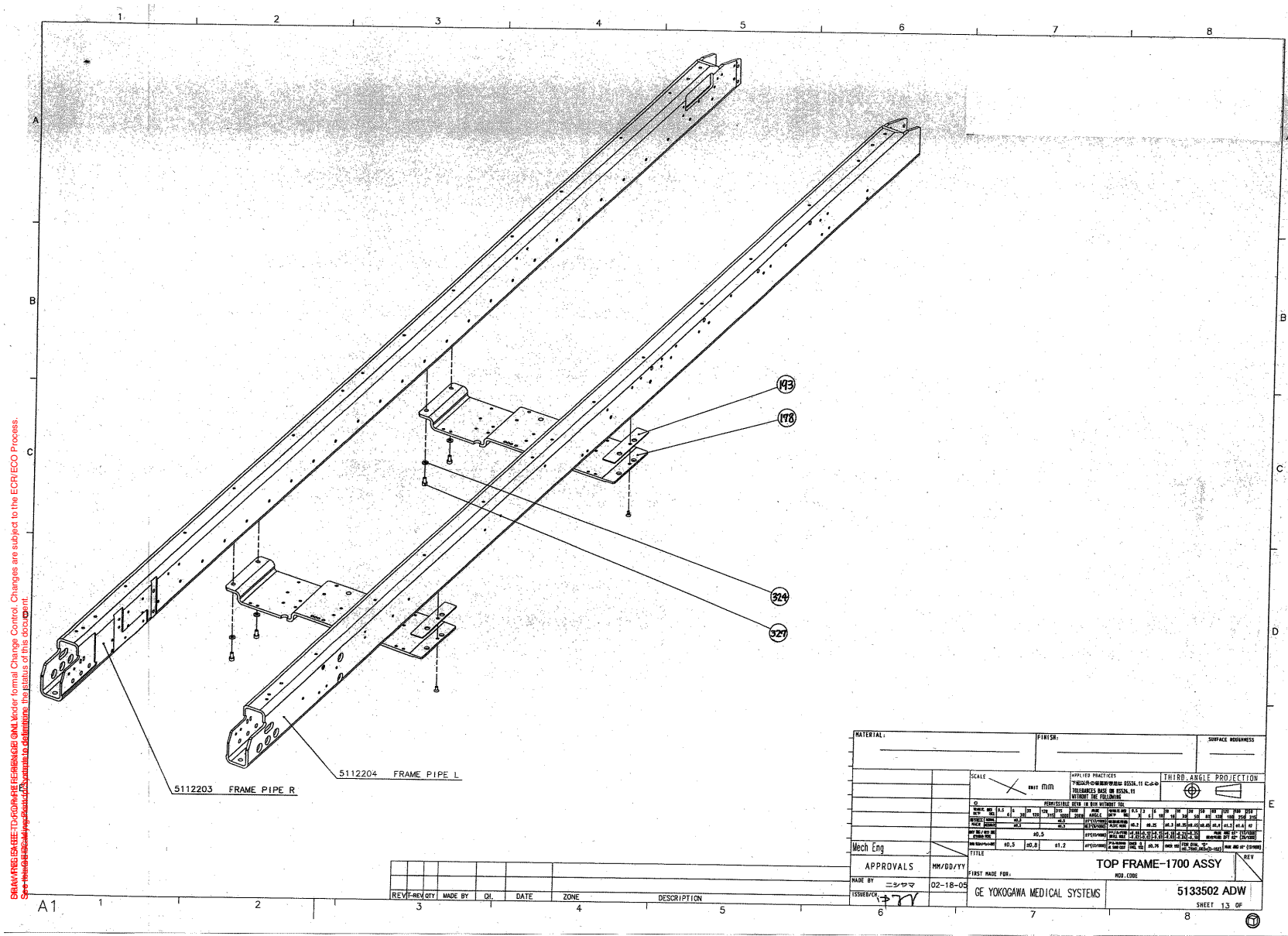
Figure 2-71 Top Frame 1700 Assembly (5133502ADW, sheet 13, rev 5)
