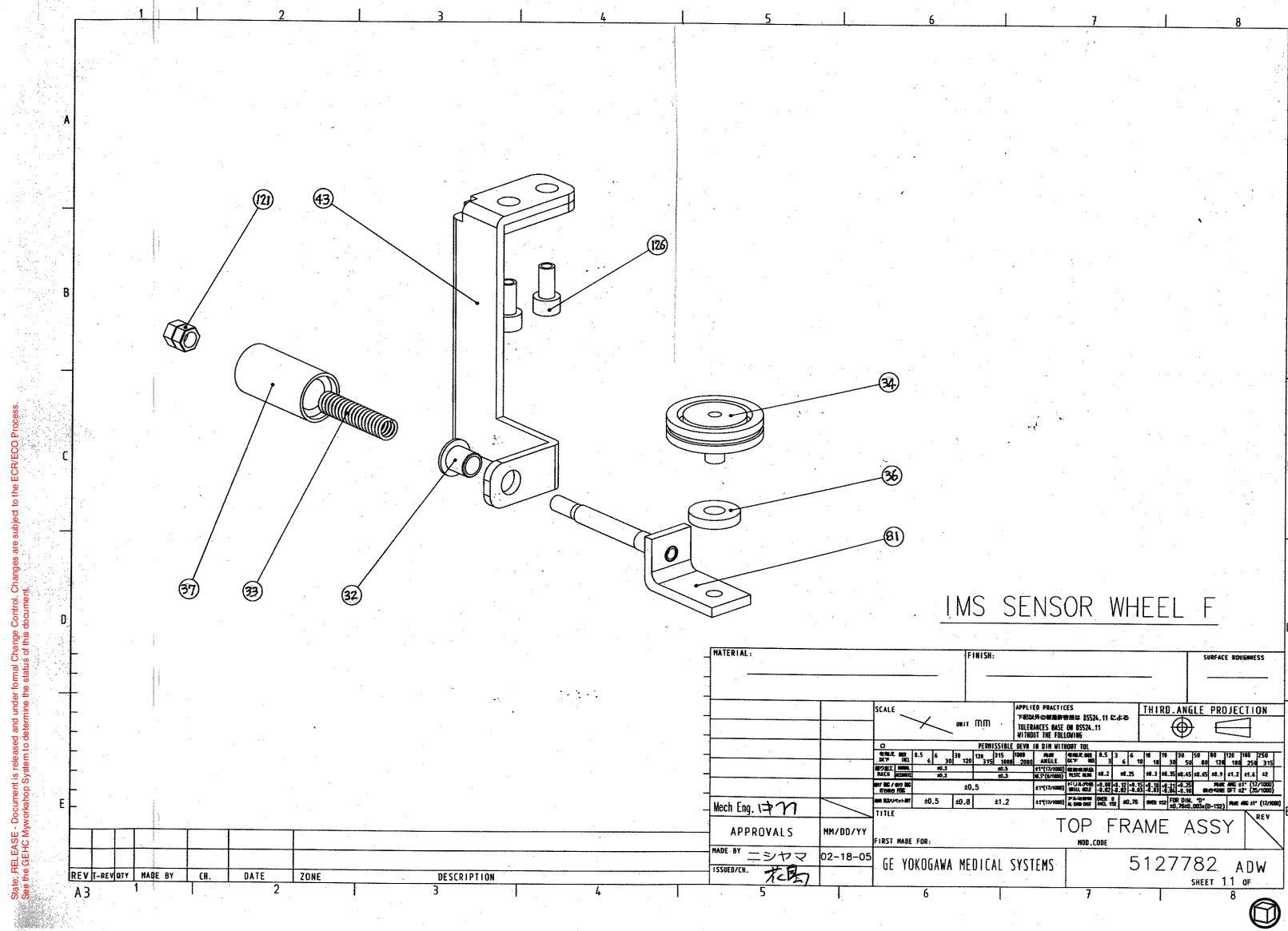
Figure 2-27 Top Frame Assembly (5127782ADW, sheet 11, rev 7)
