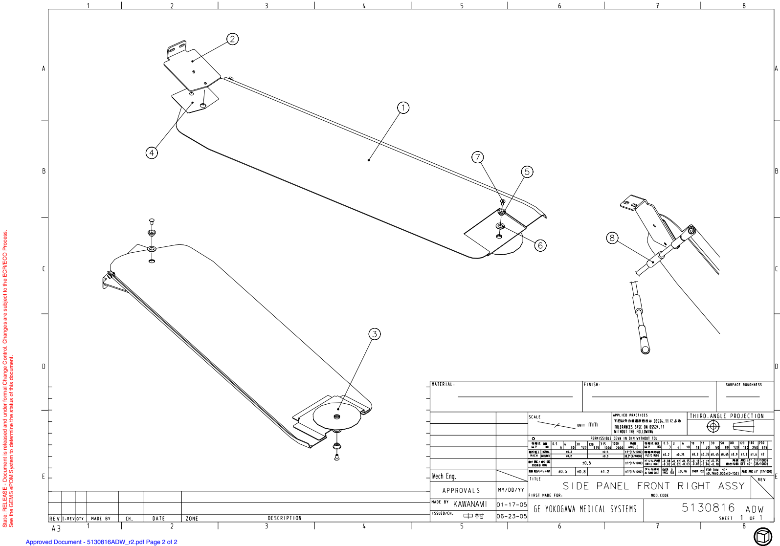
Figure 2-46 Side Panel, Front Right Assembly (5130816ADW, sheet 1, rev 2)
