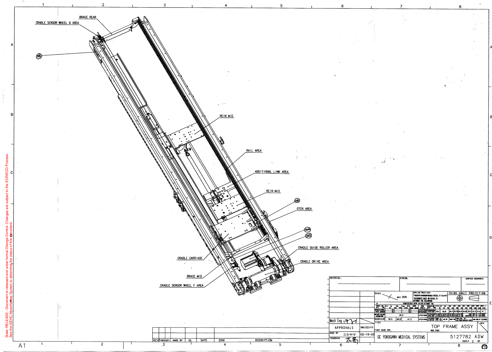
Figure 2-18 Top Frame Assembly (512778ADW2, sheet 2, rev 7)
