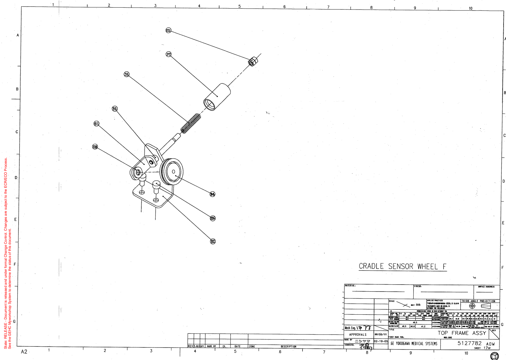
Figure 2-33 Top Frame Assembly (5127782ADW, sheet 17, rev 7)
