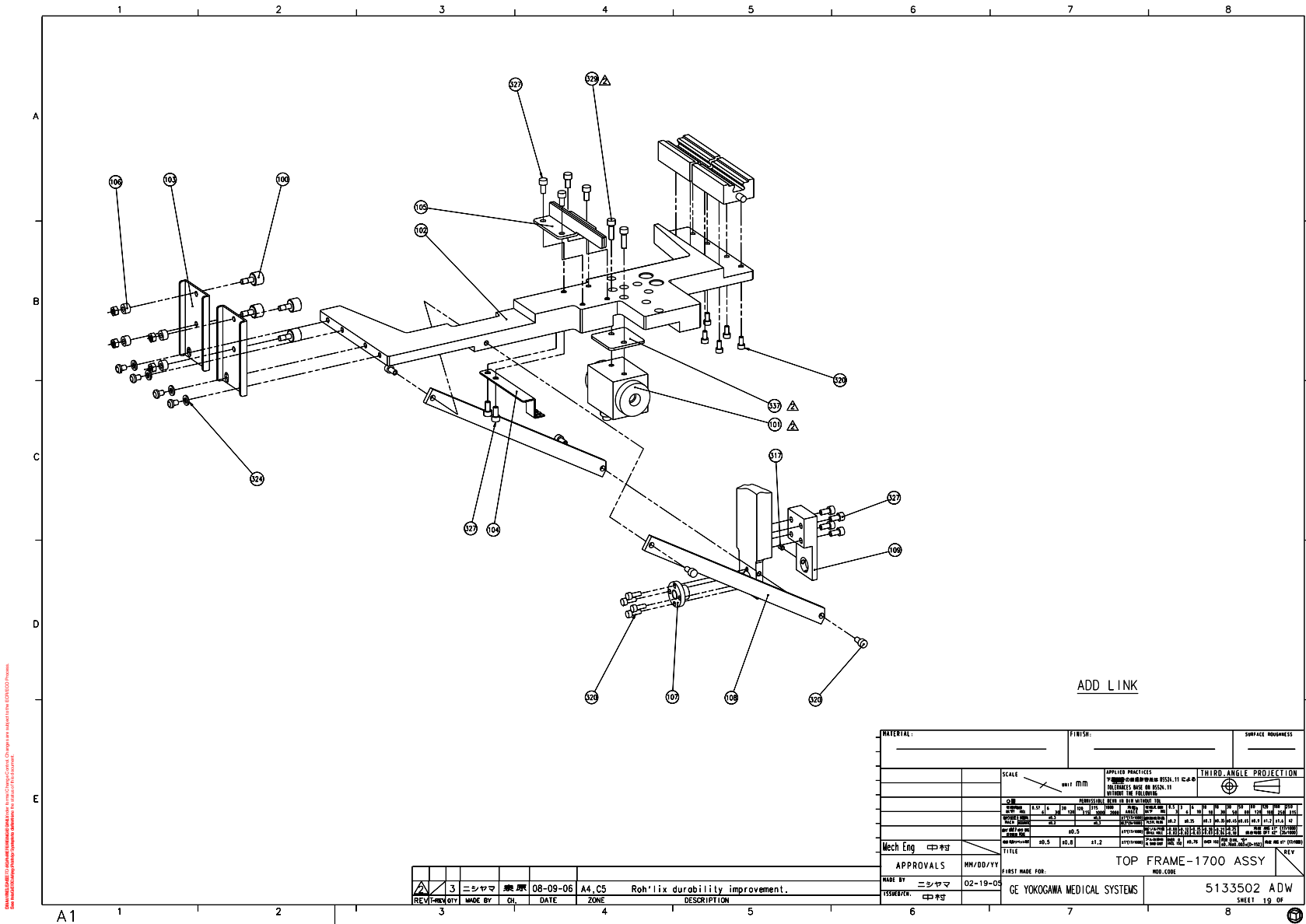
Figure 2-77 Top Frame 1700 Assembly (5133502ADW, sheet 19, rev 5)
