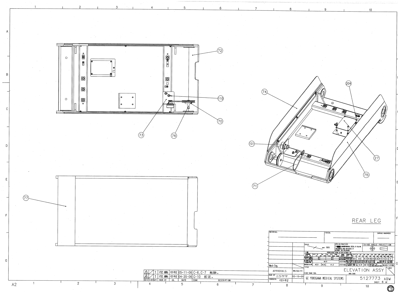
Figure 2-16 Elevation Assembly (5127773ADW, sheet 6, rev 8)
