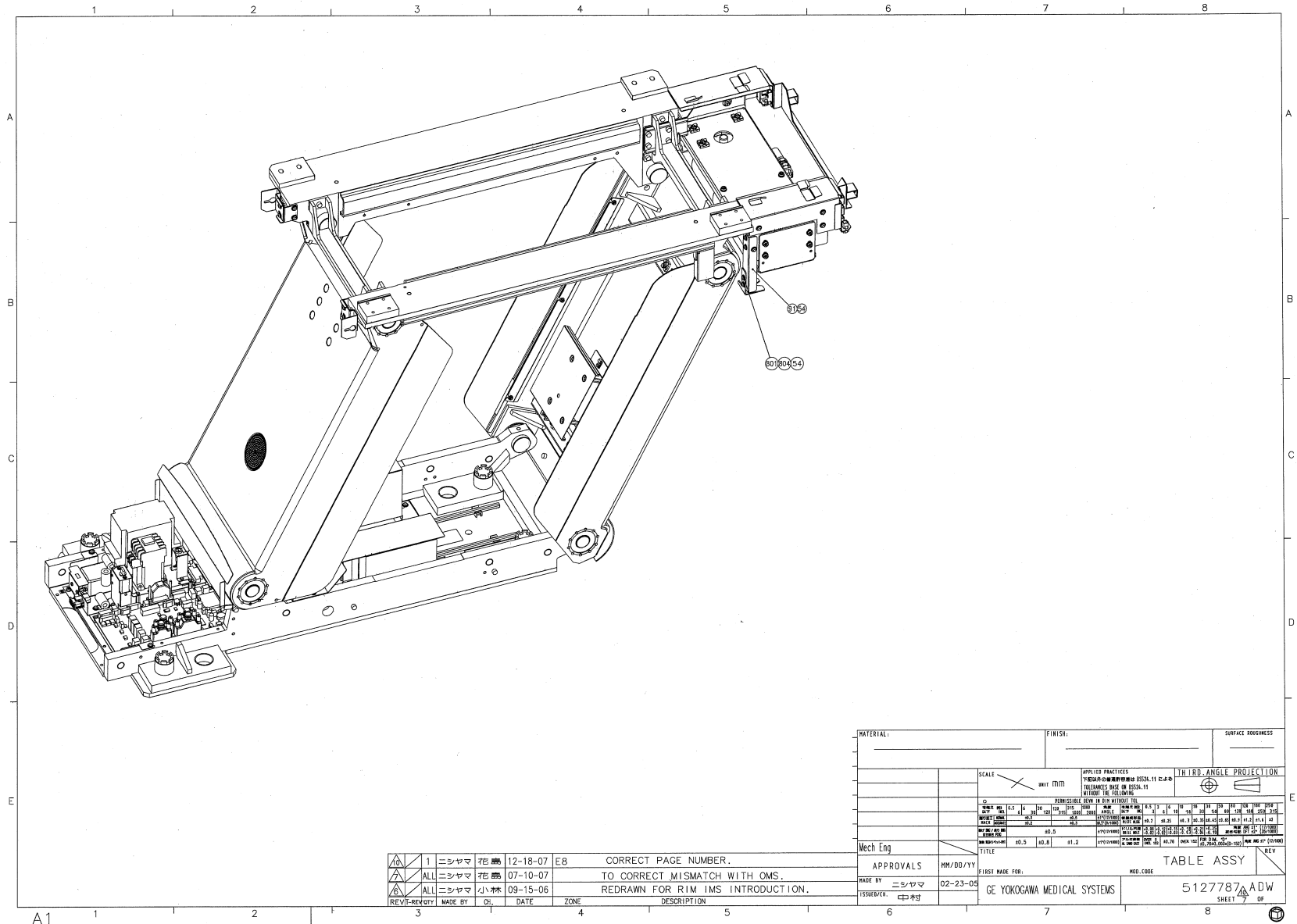
Figure 2-7 Table Assembly (5127787ADW, sheet 7, rev 10)
