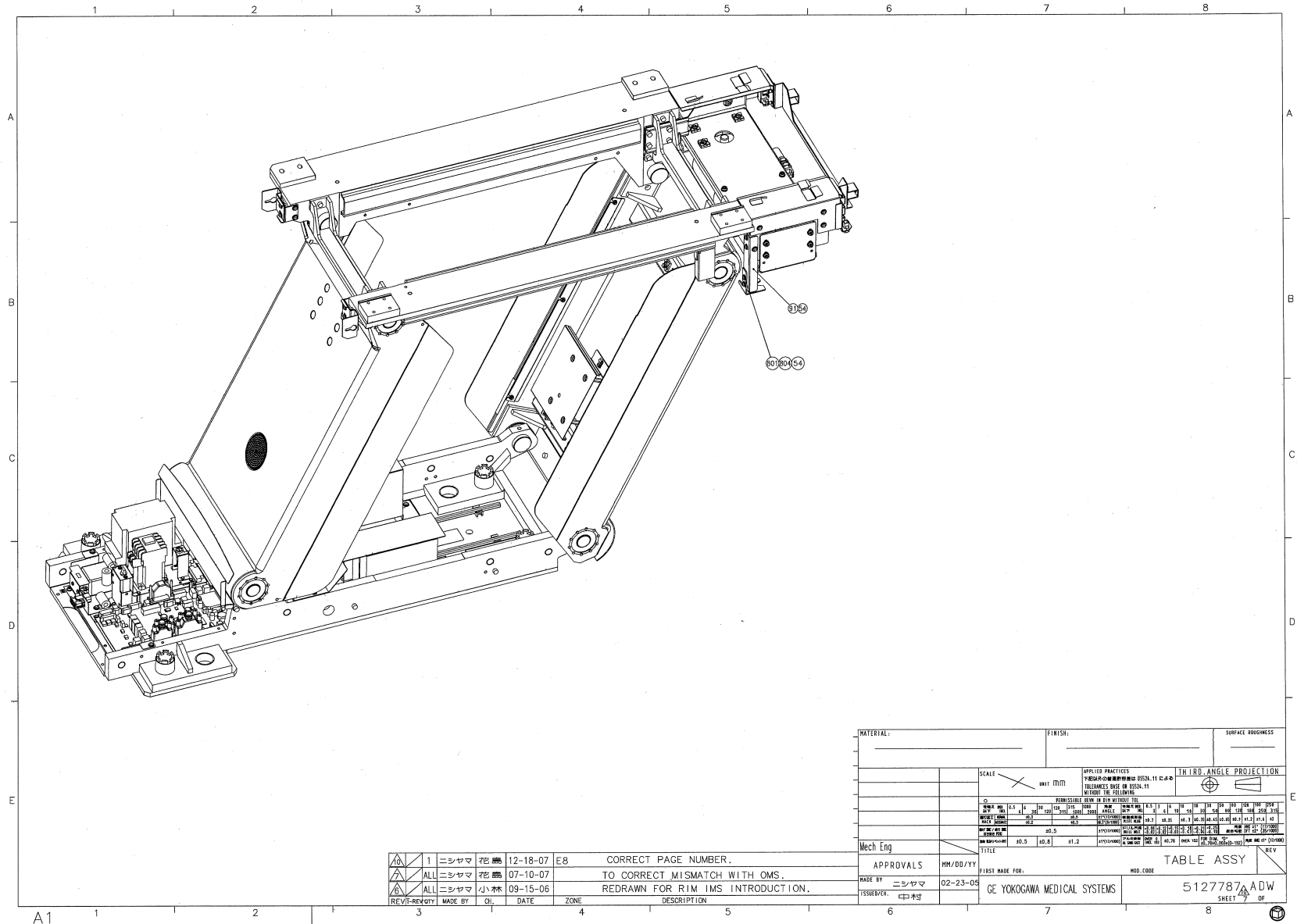
Figure 2-55 Table Assembly (5127787ADW, sheet 7, rev 10)
