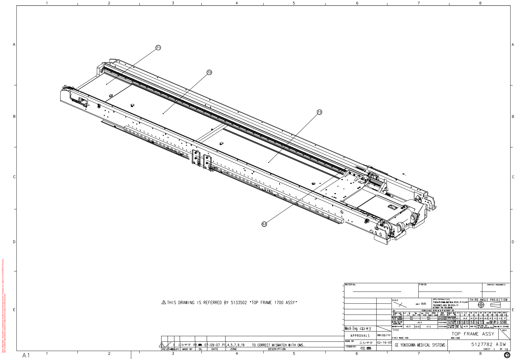
Figure 2-17 Top Frame Assembly (5127782ADW, sheet 1, rev 7)
