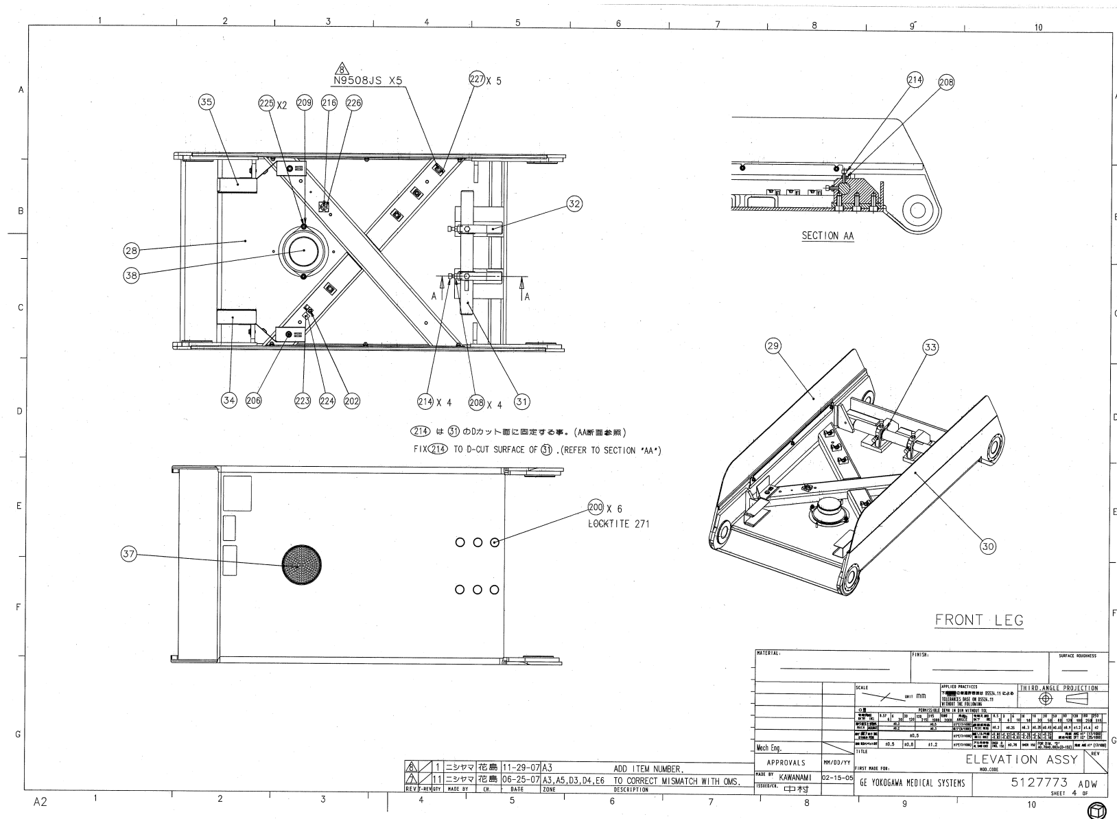
Figure 2-14 Elevation Assembly (5127773ADW, sheet 4, rev 8)
