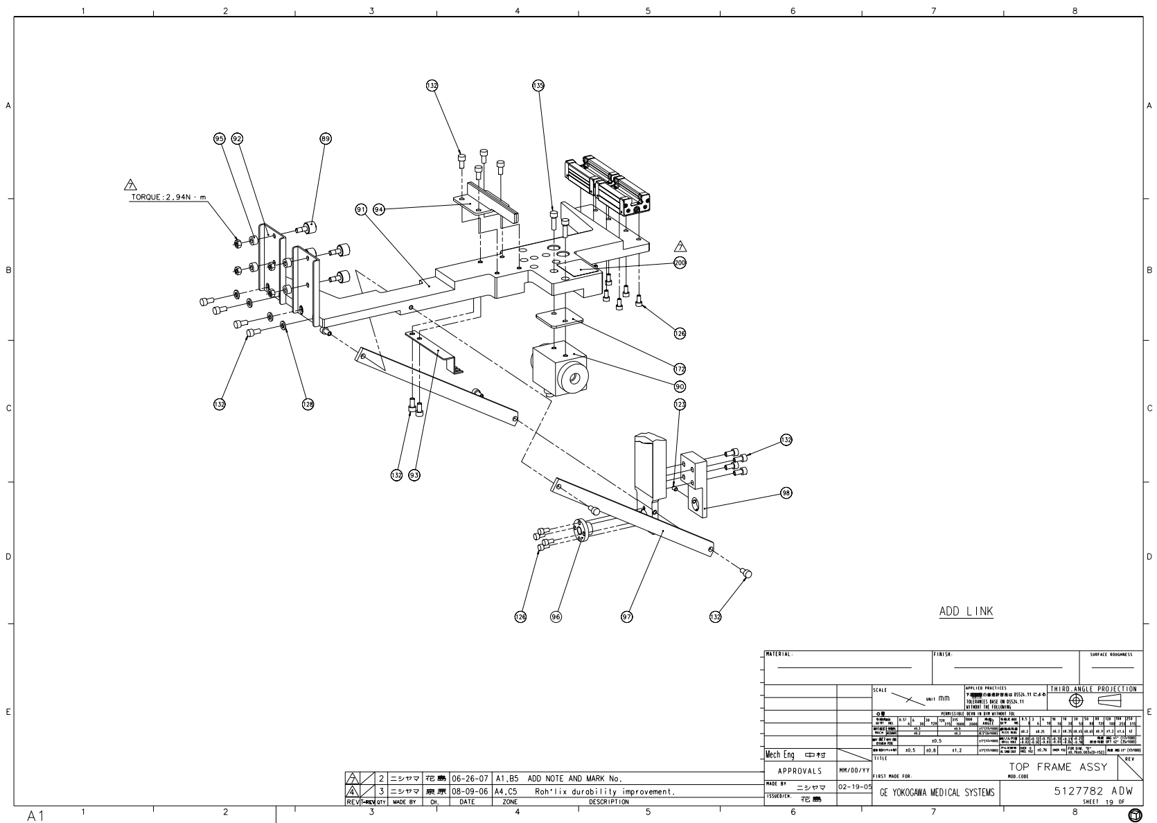
Figure 2-35 Top Frame Assembly (5127782ADW, sheet 19, rev 7)
