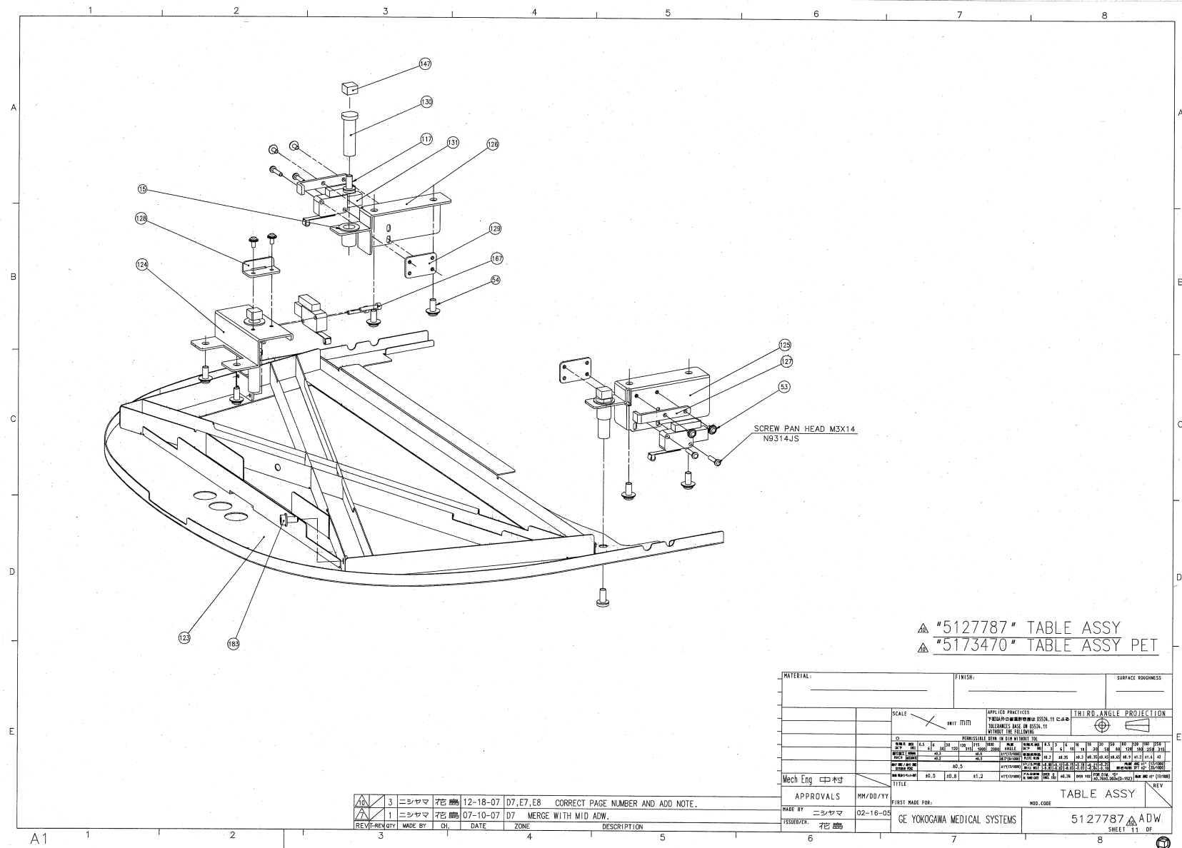
Figure 2-11 Table Assembly (5127787ADW, sheet 11, rev 10)
