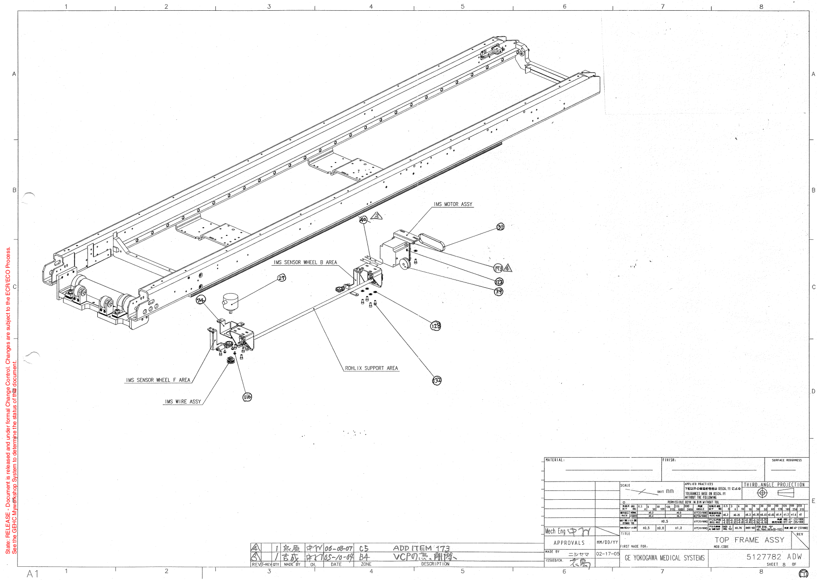
Figure 2-24 Top Frame Assembly (5127782ADW, sheet 8, rev 7)
