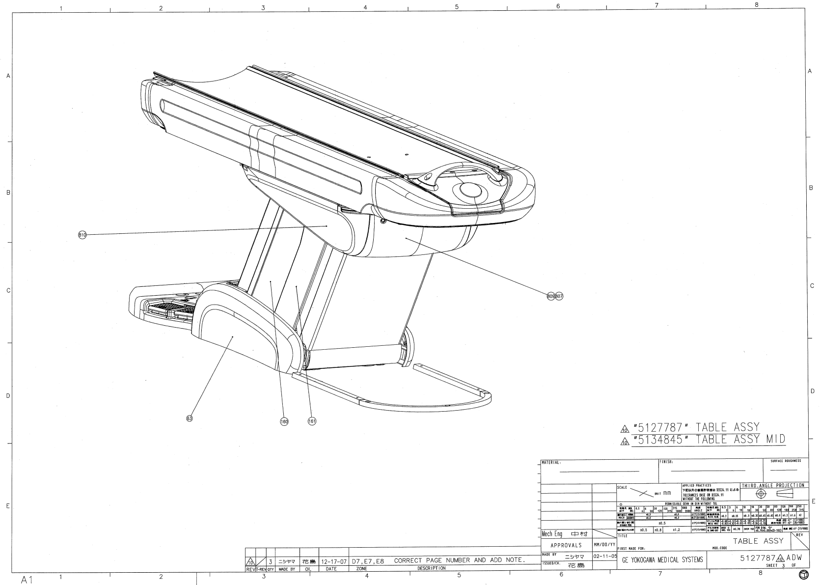
Figure 2-3 Table Assembly (5127787ADW, sheet 3, rev 10)
