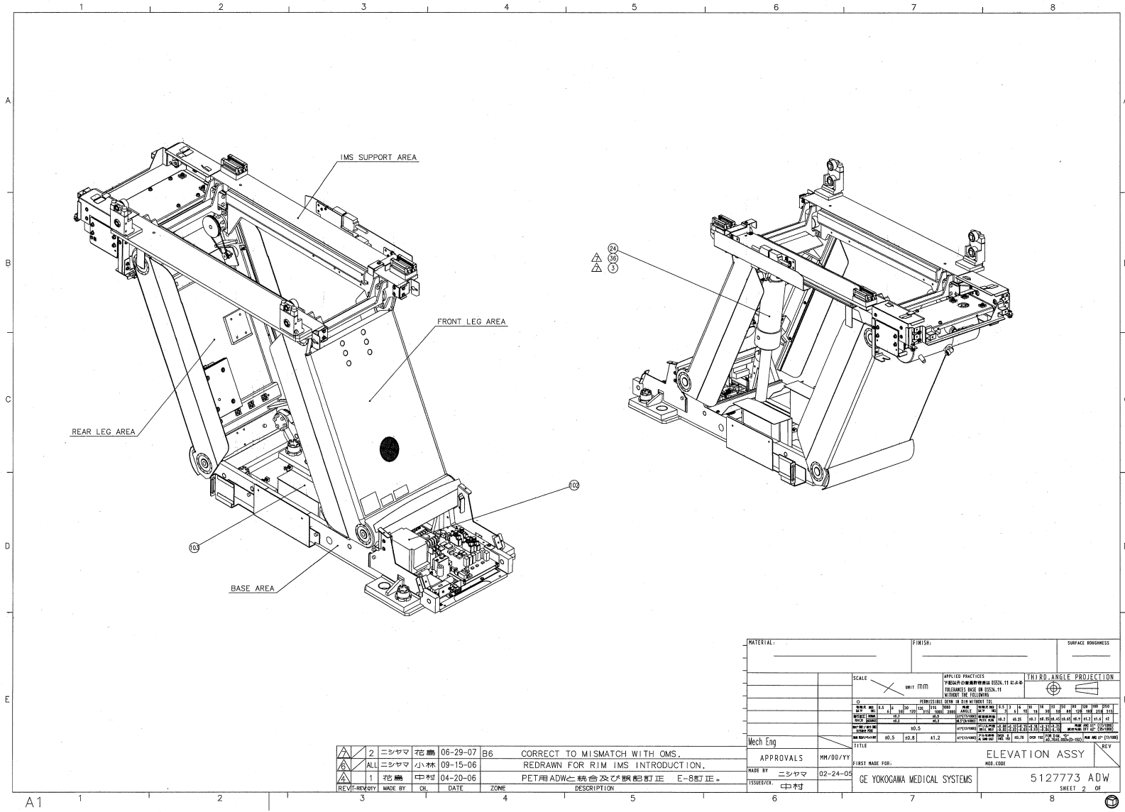
Figure 2-12 Elevation Assembly (5127773ADW, sheet 2, rev 8)
