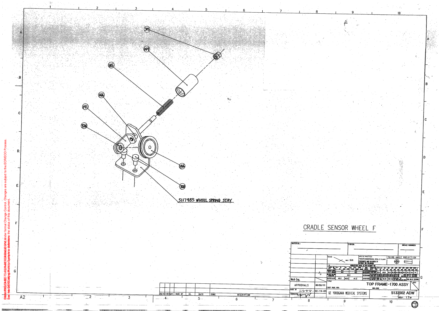
Figure 2-75 Top Frame 1700 Assembly (5133502ADW, sheet 17, rev 5)
