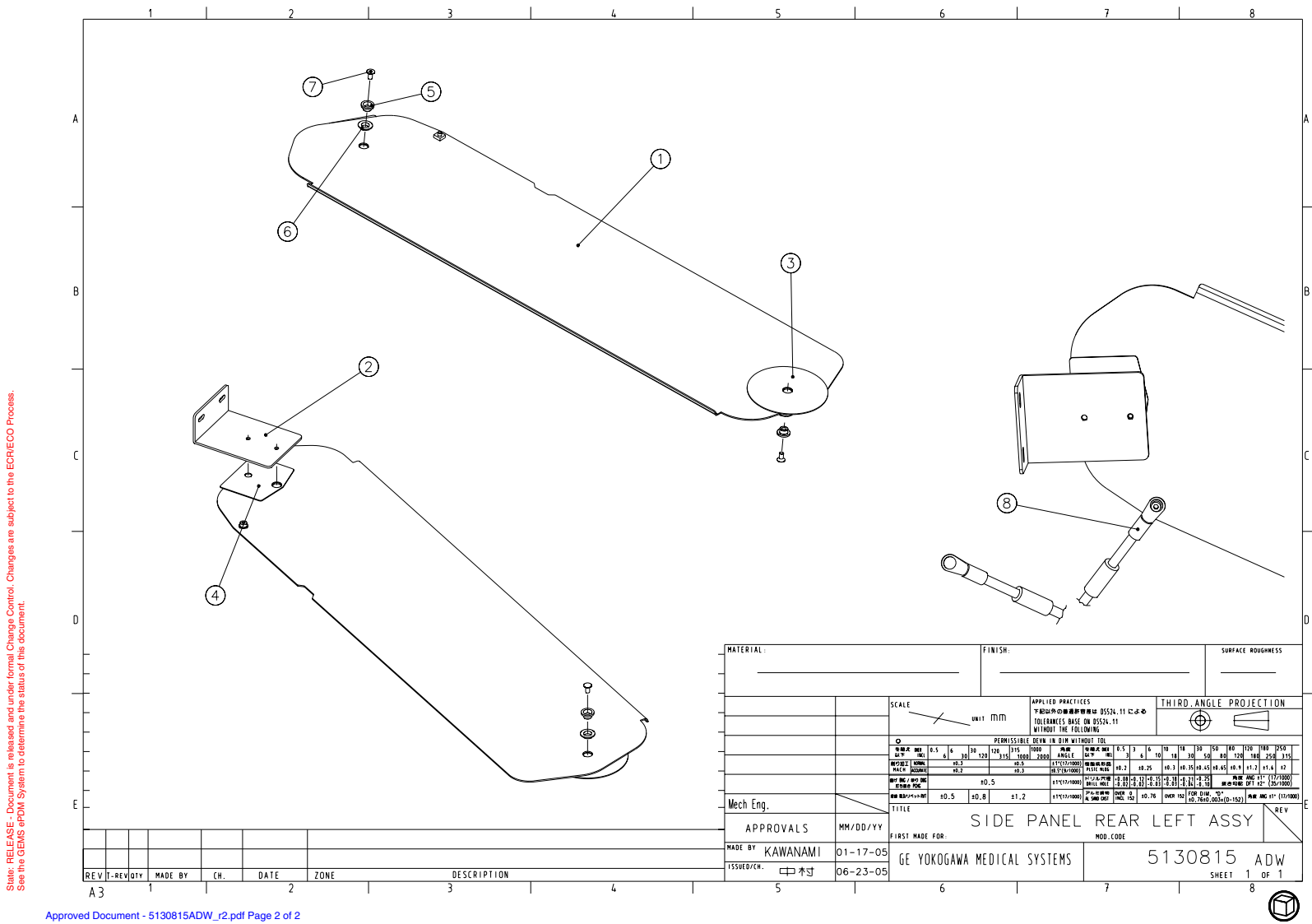
Figure 2-45 Side Panel, Rear Left Assembly (5130815ADW, sheet 1, rev 2)
