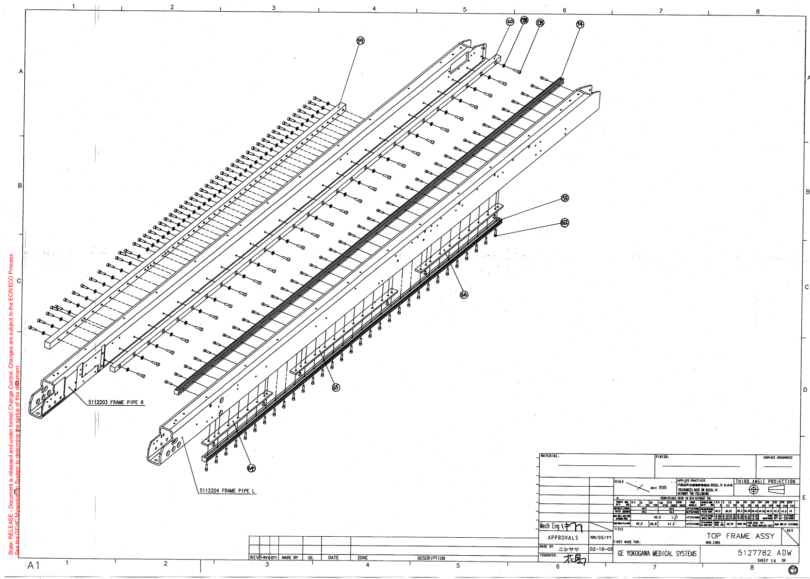
Figure 2-30 Top Frame Assembly (5127782ADW, sheet 14, rev 7)
