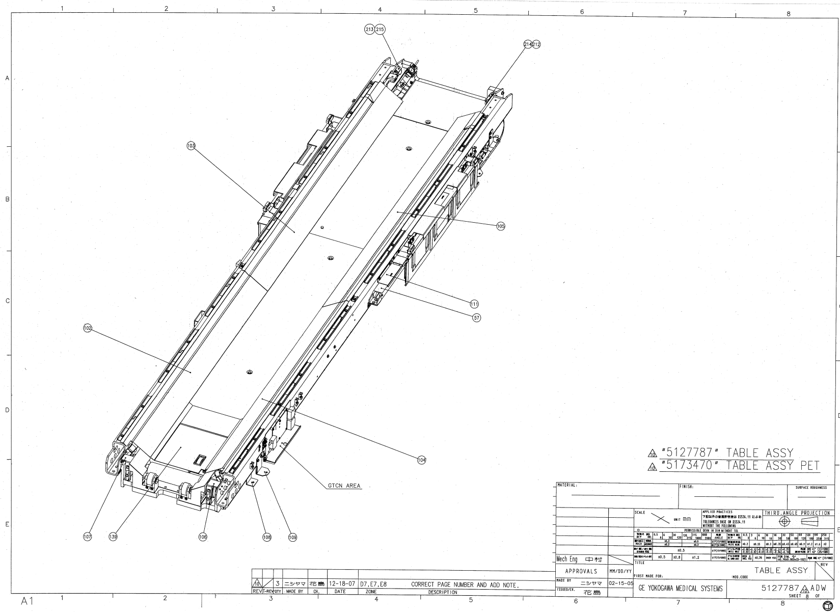
Figure 2-8 Table Assembly (5127787ADW, sheet 8, rev 10)
