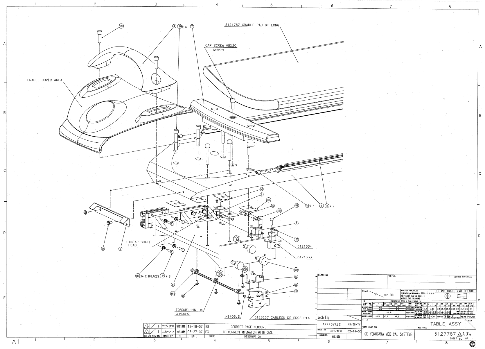
Figure 2-57 Table Assembly (5127787ADW, sheet 10, rev 10)
