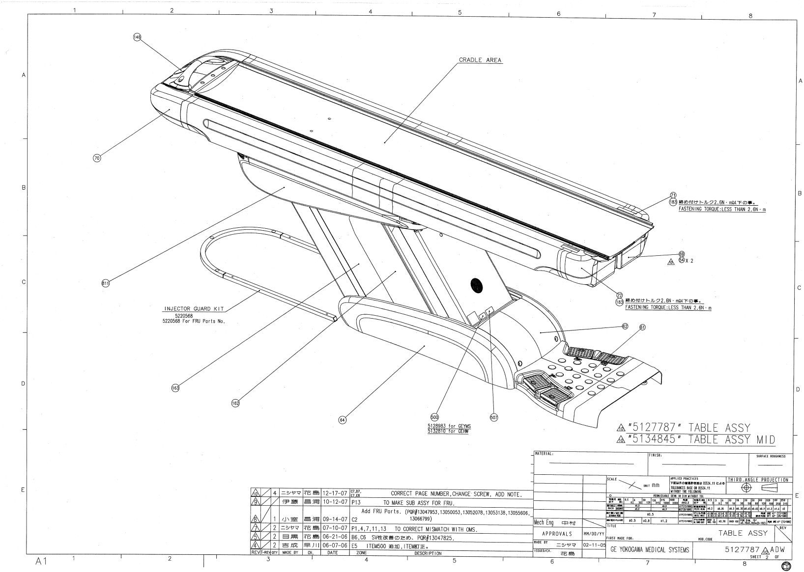
Figure 2-50 Table Assembly (5127787ADW, sheet 2, rev 10)
