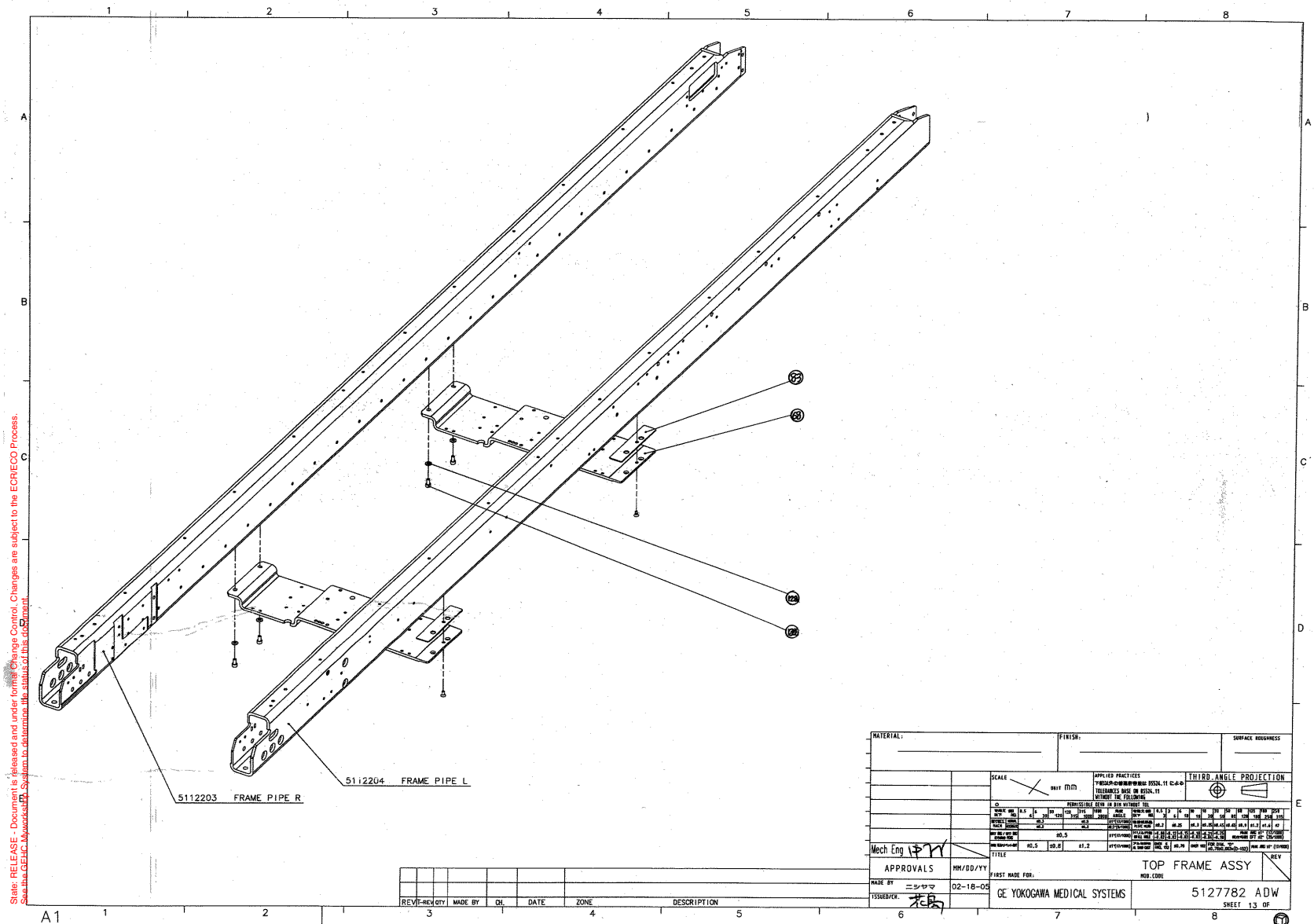
Figure 2-29 Top Frame Assembly (5127782ADW, sheet 13, rev 7)
