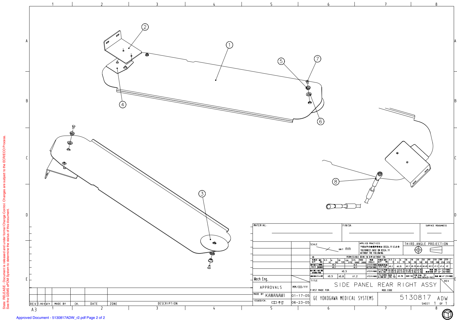
Figure 2-47 Side Panel, Right Rear Assembly (5130817ADW, sheet 1, rev 2)
