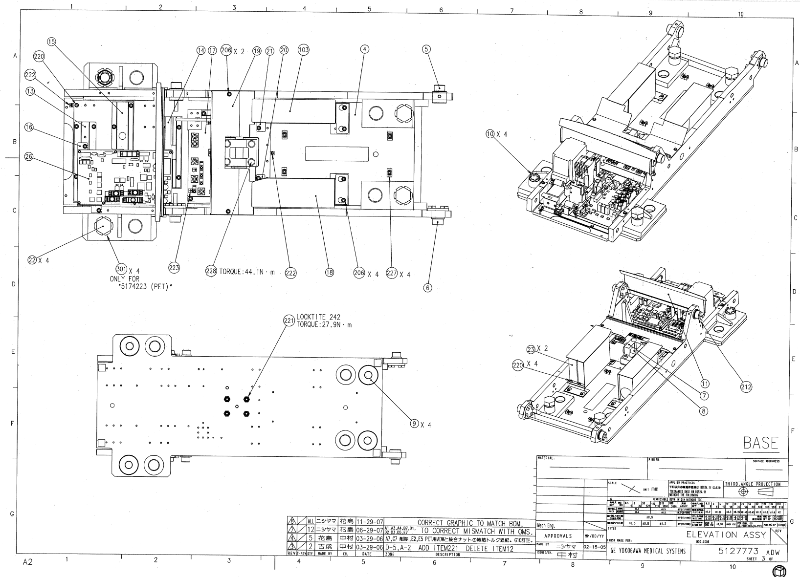
Figure 2-13 Elevation Assembly (5127773ADW, sheet 3, rev 8)
