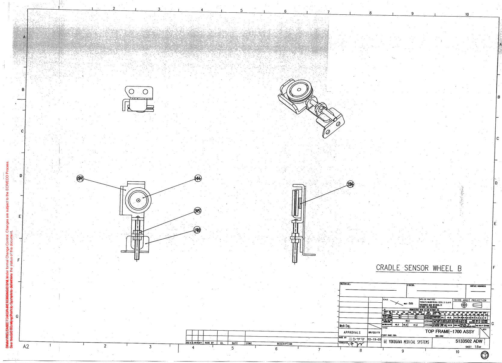
Figure 2-76 Top Frame 1700 Assembly (5133502ADW, sheet 18, rev 5)
