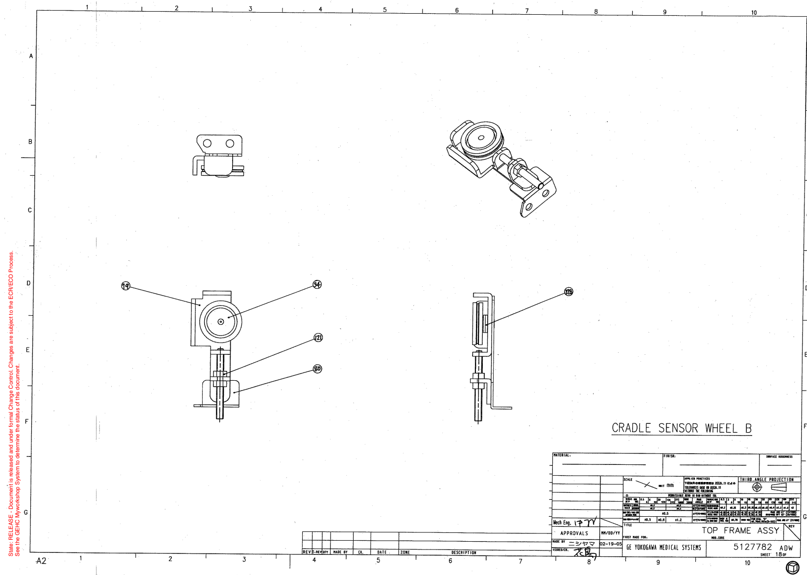
Figure 2-34 Top Frame Assembly (5127782ADW, sheet 18, rev 7)
