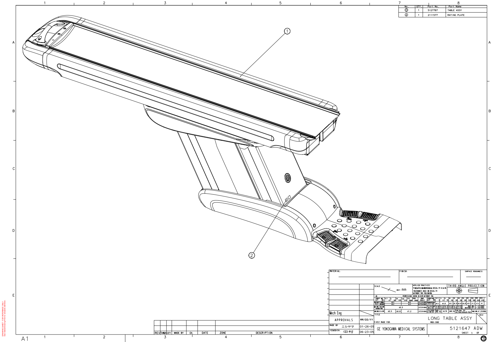
Figure 2-1 Positioning GT LONG TABLE ASSY (5121647ADW, sheet 1, rev 4)
