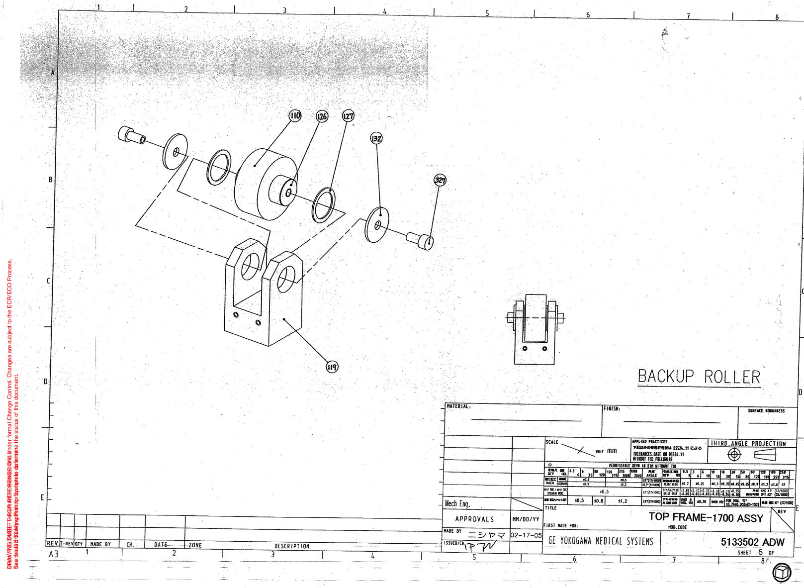
Figure 2-64 Top Frame 1700 Assembly (5133502ADW, sheet 6, rev 5)
