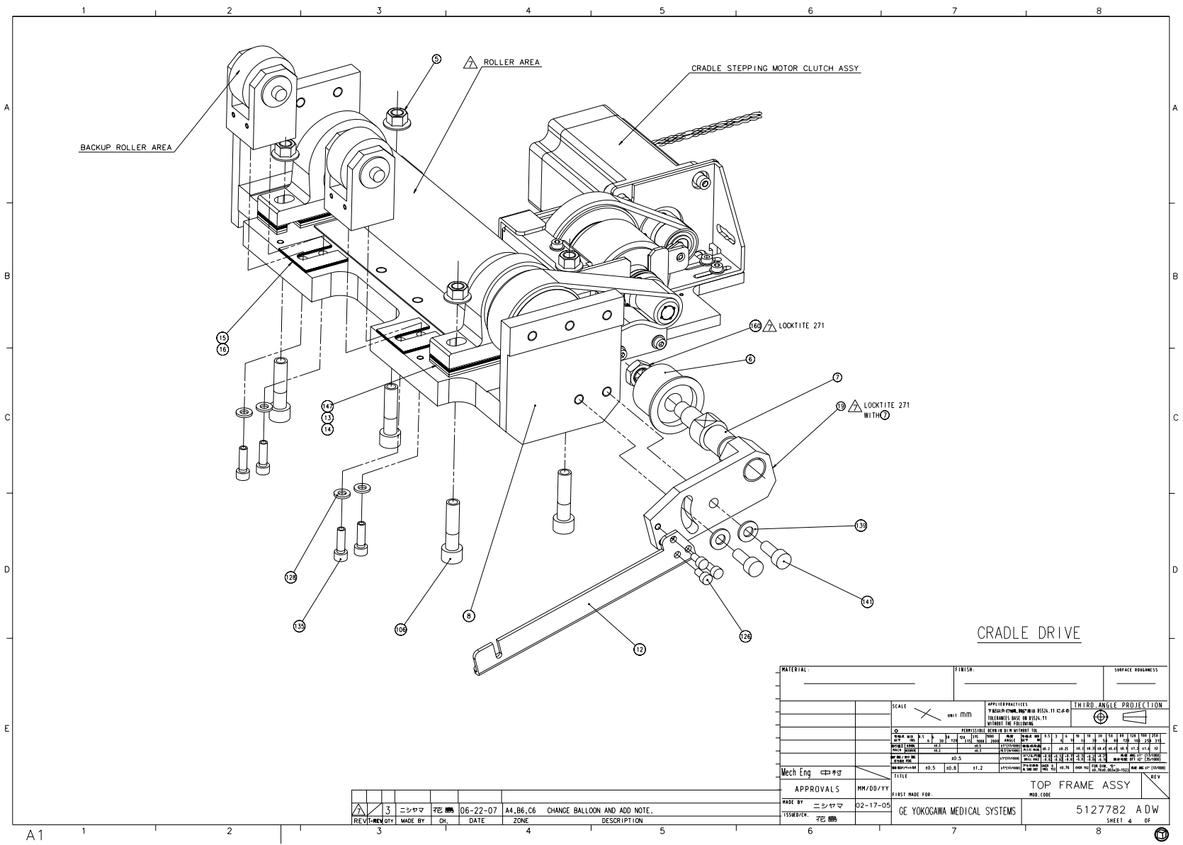
Figure 2-20 Top Frame Assembly (5127782ADW, sheet 4, rev 7)
