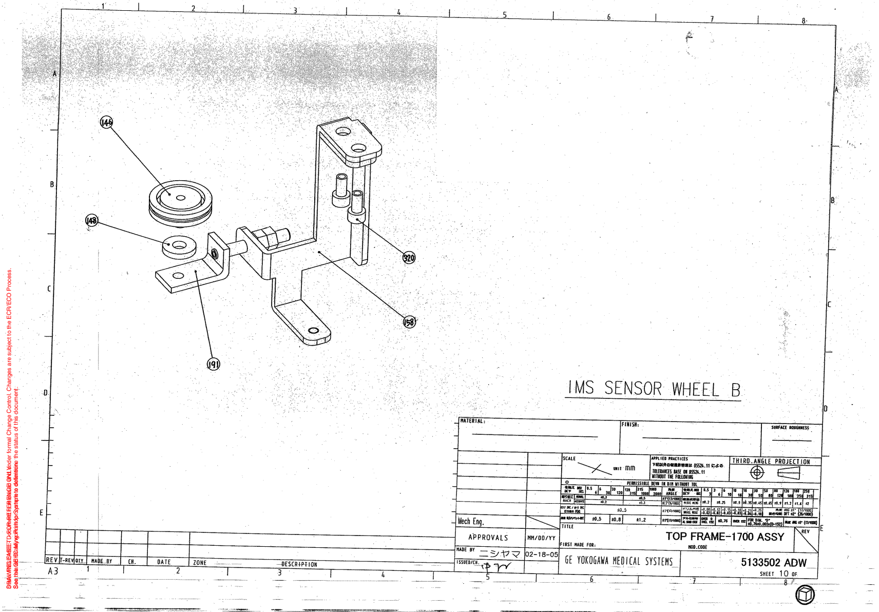
Figure 2-68 Top Frame 1700 Assembly (5133502ADW, sheet 10, rev 5)
