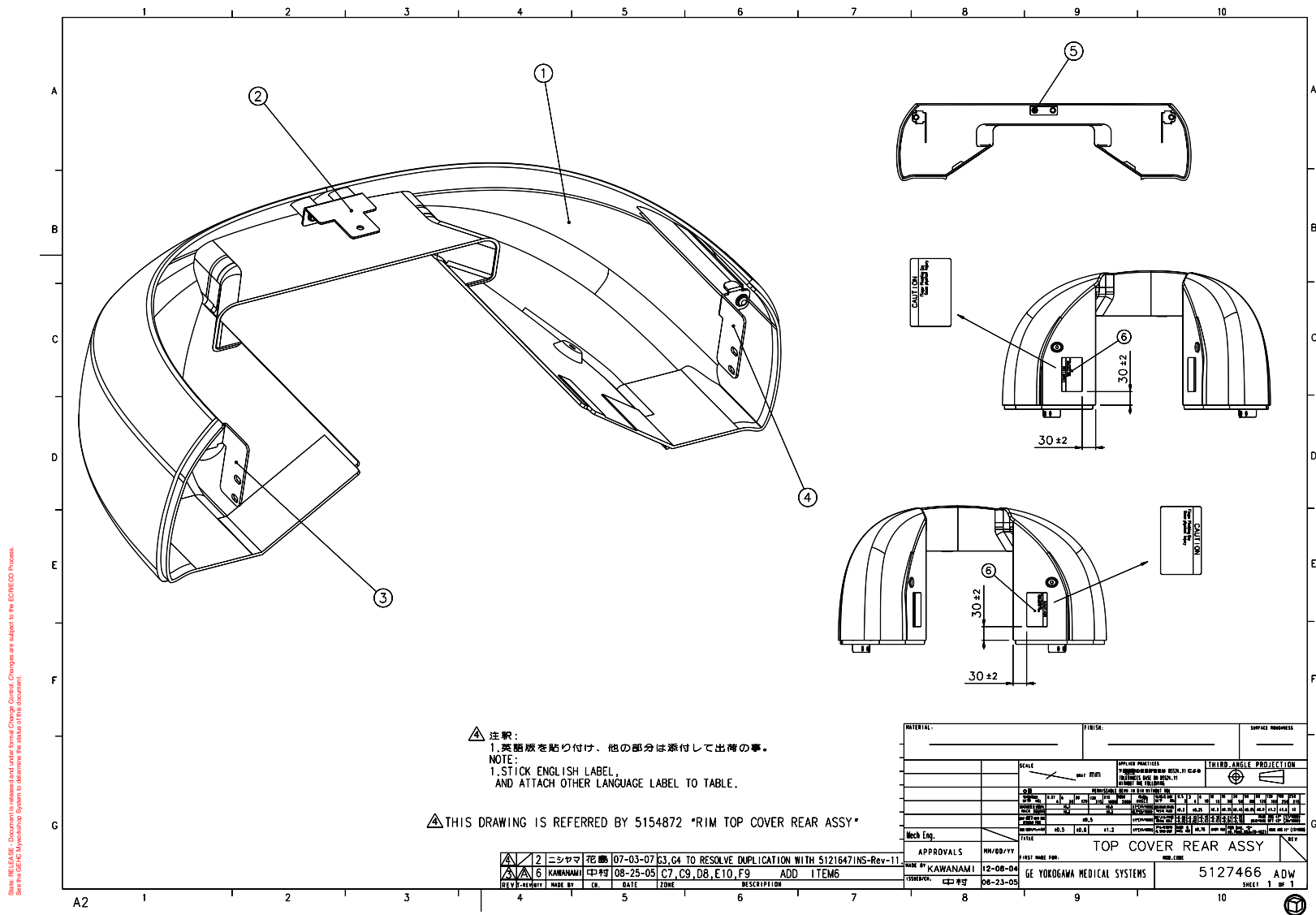
Figure 2-41 TOP COVER REAR ASSY (5127466ADW, sheet 1, rev 4)
